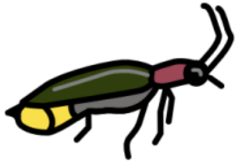
fireflies
